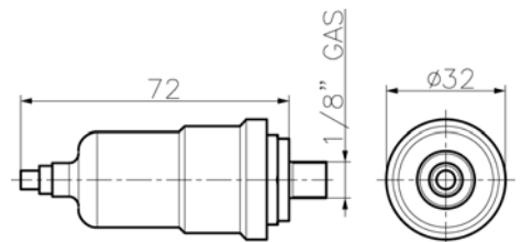
Manostat with exchanging contacts Gauging: 1.5 bar - L1 type
